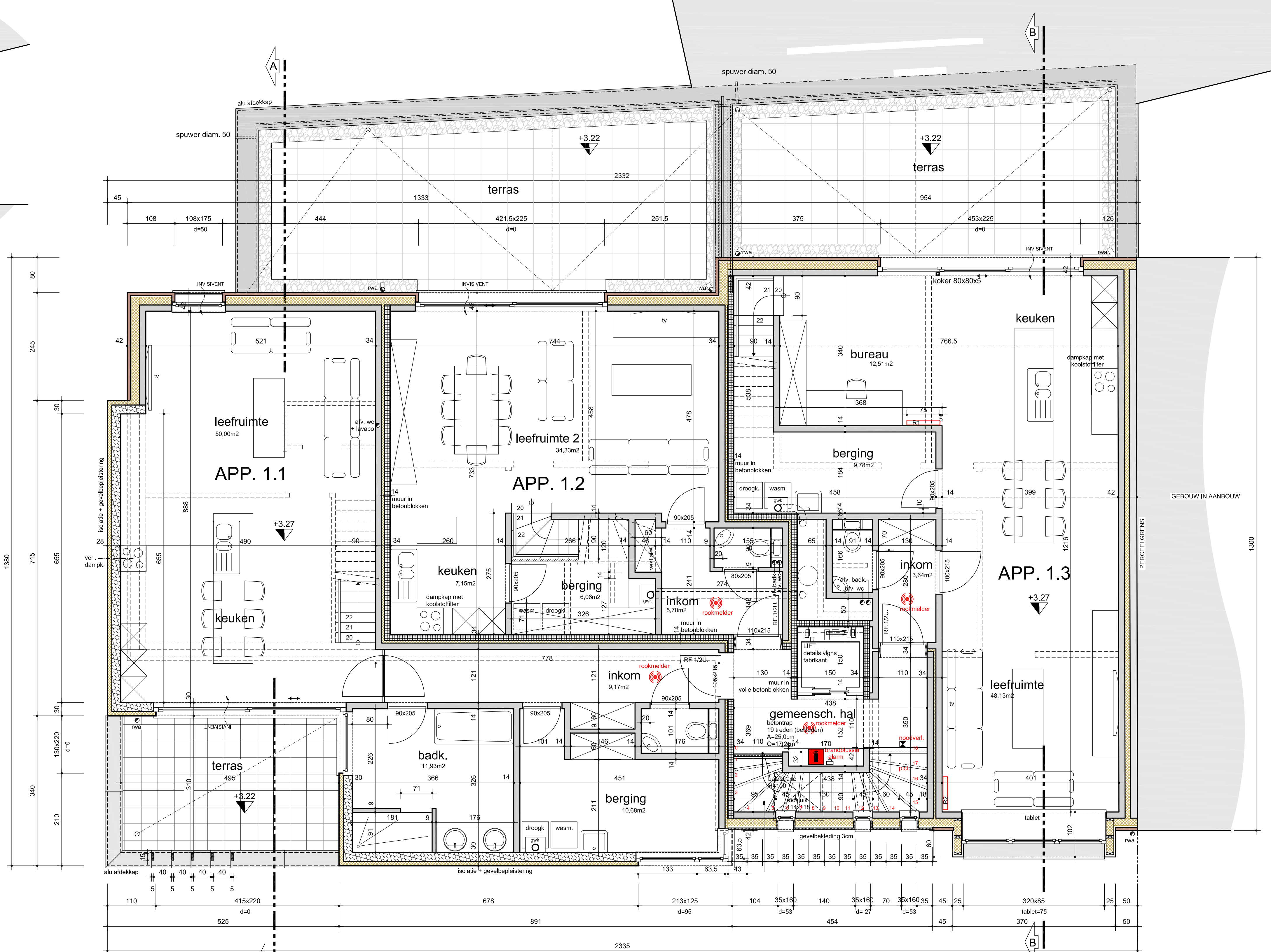
VERDIEPING 1 (peil +3.27) 1/50
