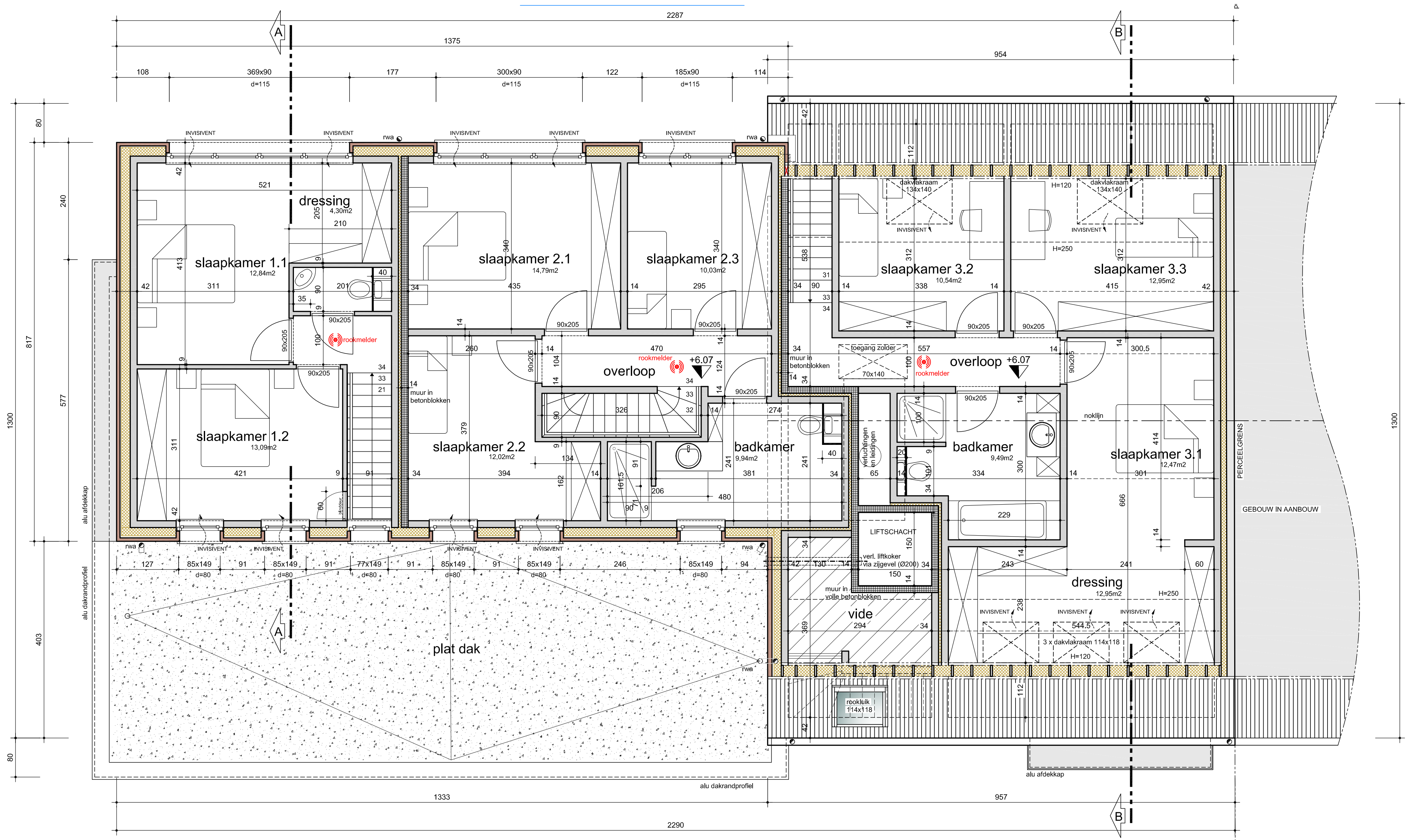
VERDIEPING 2 (peil +6.07) 1/50
